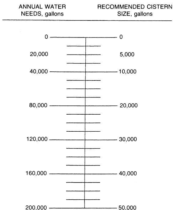
Figure 4. Cistern size based on a storage capacity equal to 1/4 of the annual water needs or a three-month supply of stored water. (Source: Midwest Plan Service, Iowa State Univ., 1968. Private Water Systems. p. 15.)
