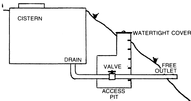
Figure 10. Plan for cleanout drain and control valve.
