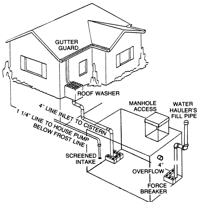
Figure 1. Typical roof-catchment cistern system. (Source: Water Filtration Co. customer information brochure. Water Filtration Co., 108B Industry Rd., Marietta, Ohio 45750.)
