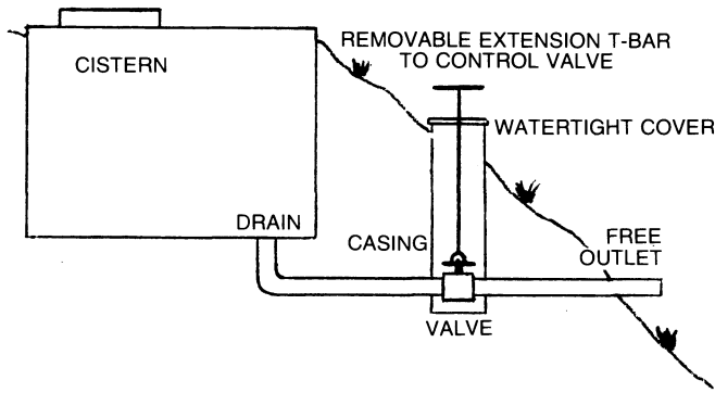
Figure 9. Plan for cleanout drain and control valve.
