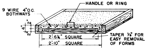
Figure 7. Section thru form for manhole cover.
