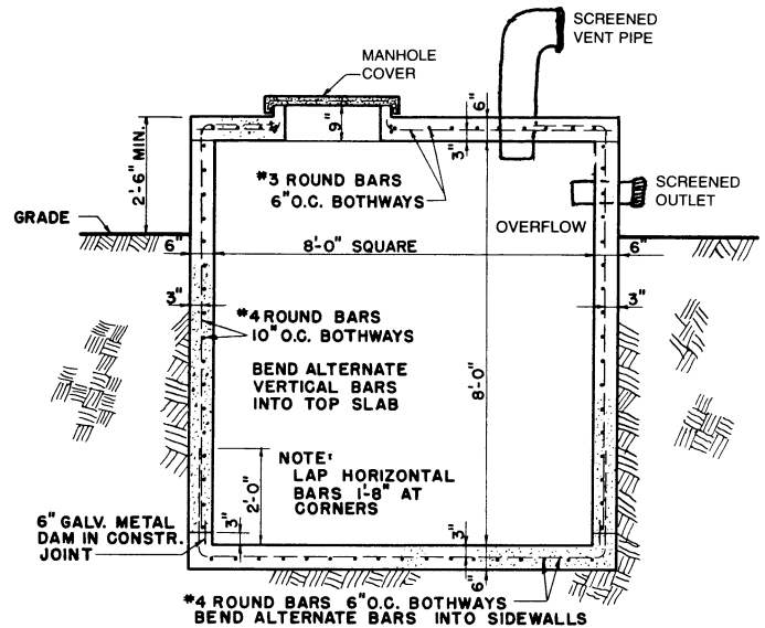
Figure 8. Cross section of 8' x 8' cistern showing overflow pipe, manhole, and vent pipe.
