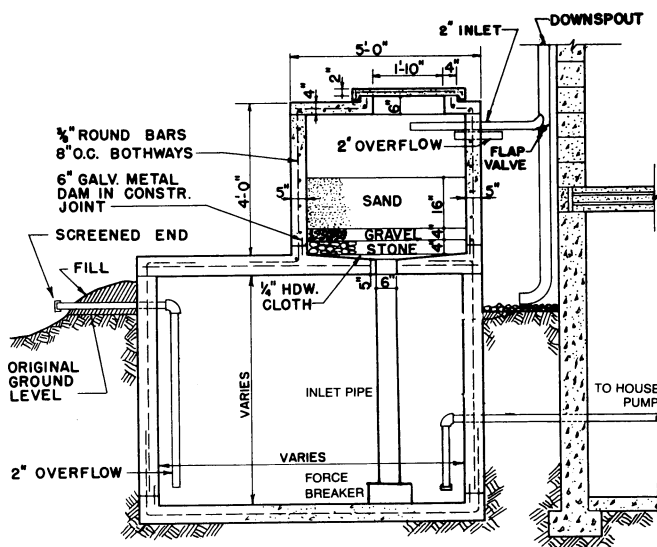
Figure 6. Cross section of concrete cistern with filter (Source: PSU Ag Ext. Service, Order #800-87 Concrete Cisterns)
