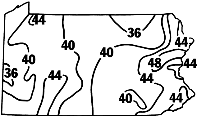
Figure 2. Average annual precipitation for Pennsylvania (inches)
