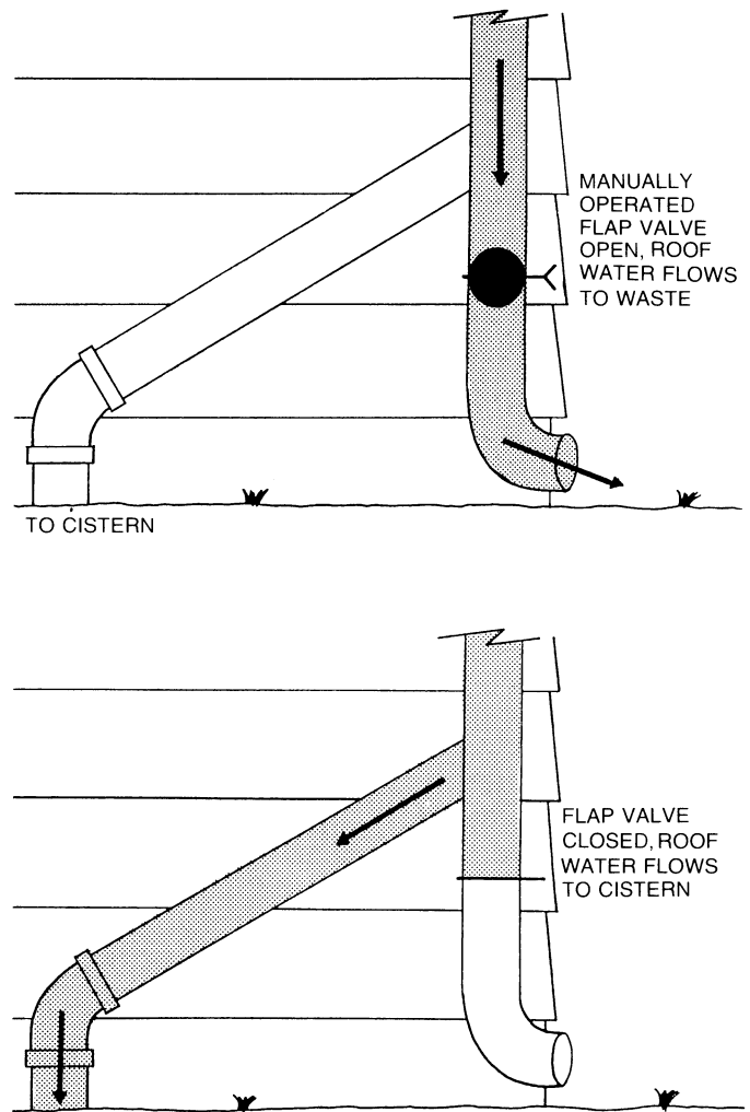
Figure 12. A simple roof-wash diverter.
