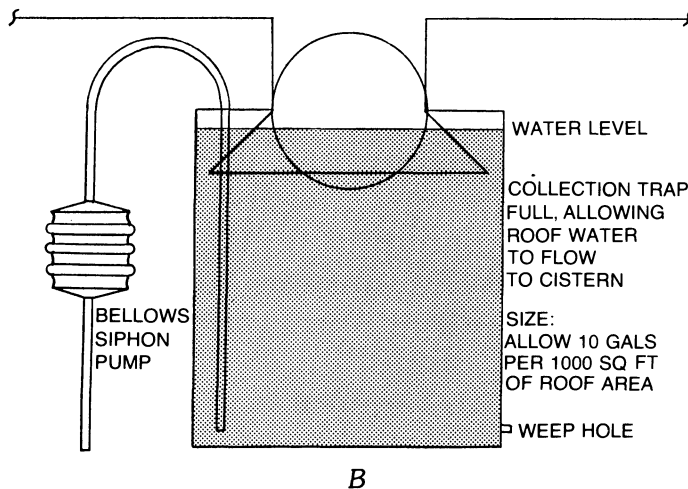
Figure 13. Automatic roof-wash diverter.
